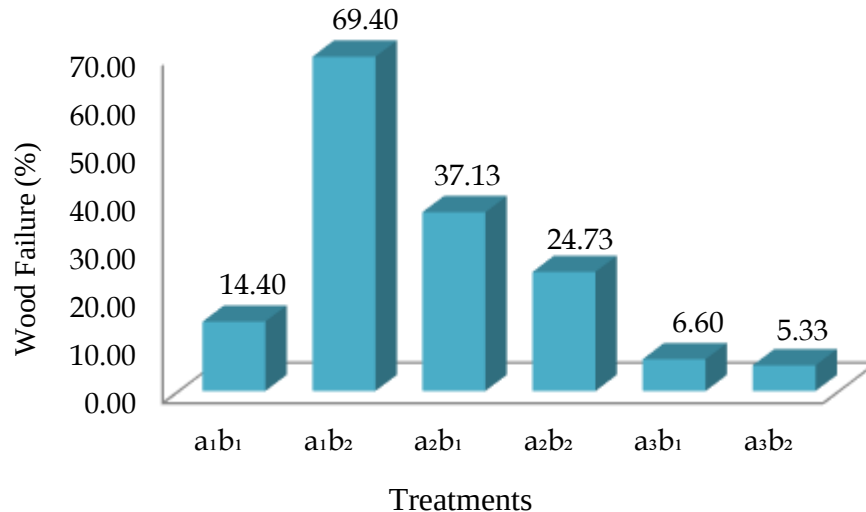
Figure 3. Mean Percentage of Wood Failure (%WF)
